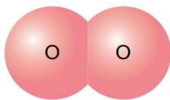
Khí oxygen
